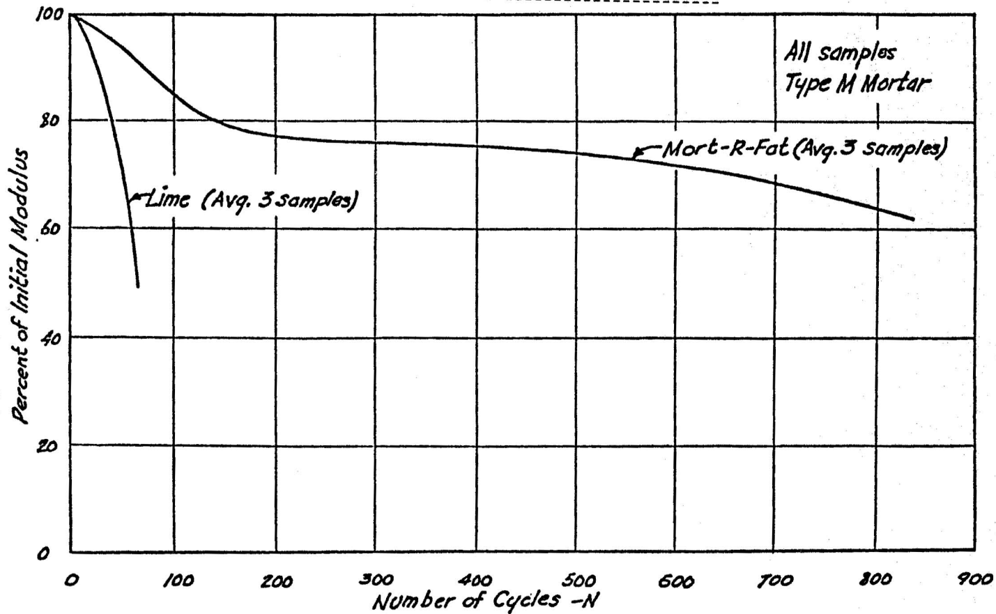
Fig. 1 Results of Freeze-Thaw Tests on Prisms of Mortar prepared with lime and with Mort-R-Fat (Tests conducted by L.H. Shifley, University of Nevada, Reno).
